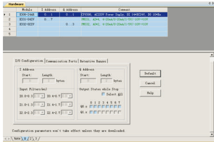
Hardware Configuration
